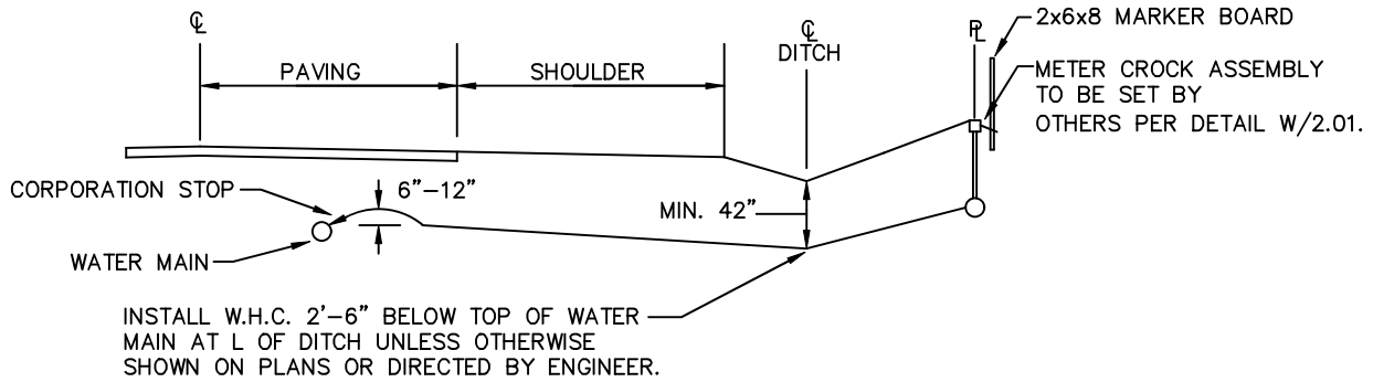
PARTIAL WIDTH GRADING (CUT SECTION)
