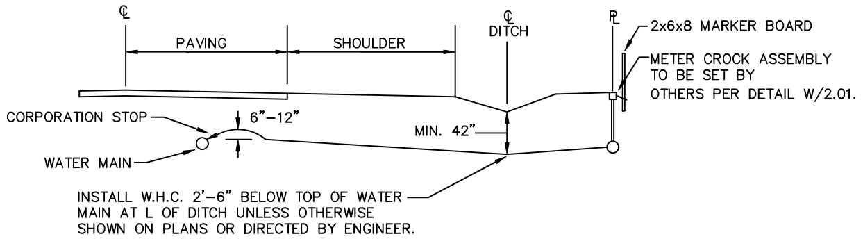
FULL WIDTH GRADING
