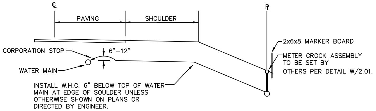
PARTIAL WIDTH GRADING (FILL SECTION)
