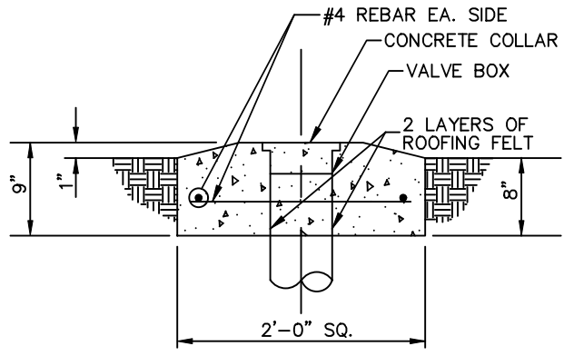
CONCRETE VALVE BOX COLLAR
