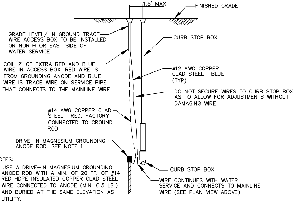
WATER SERVICE – SECTION VIEW NOT TO SCALE
