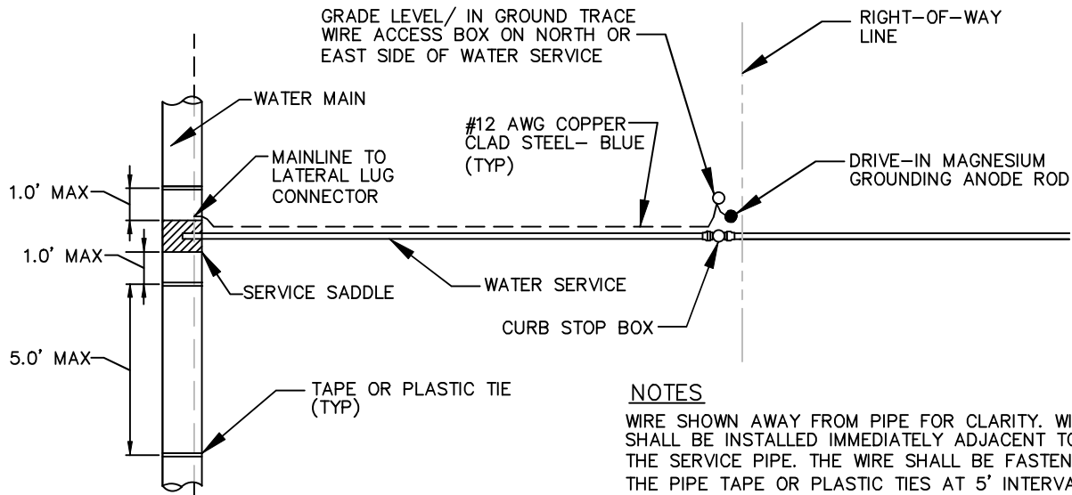
WATER SERVICE – PLAN VIEW NOT TO SCALE
