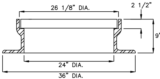
FRAME SECTION
