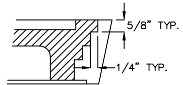
DETAIL OF PICKHOLE
