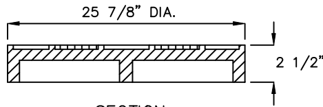
SECTION
