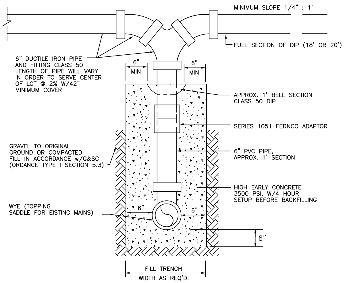
TYPICAL DROP HOUSE CONNECTION
