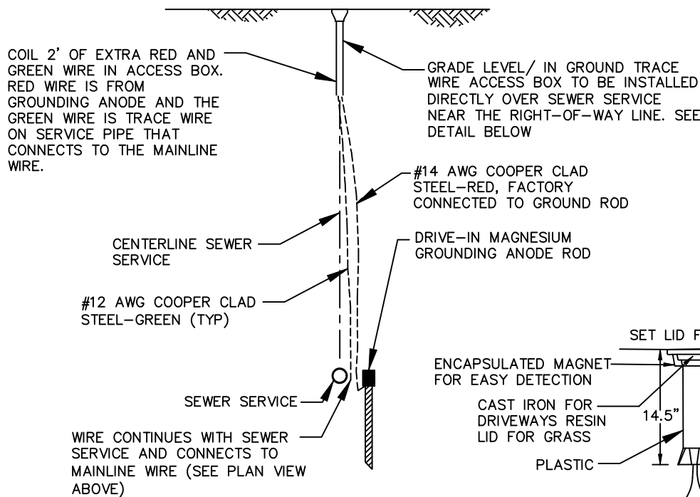
SEWER SERVICE - SECTION VIEW NOT TO SCALE
