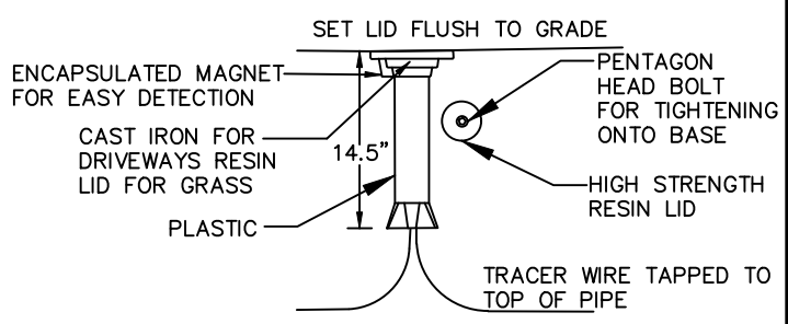
TRACER WIRE ACCESS DETAIL NOT TO SCALE
