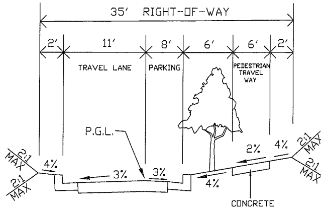
CLOSED SECTION ONE WAY
