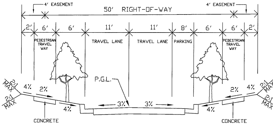
CLOSED SECTION TWO WAY - ONE SIDED PARKING
