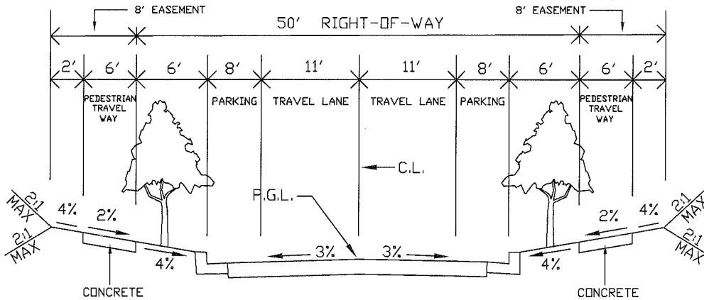
CLOSED SECTION TWO WAY - TWO SIDED PARKING
