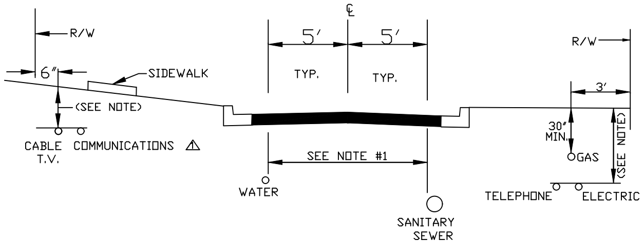
LOCATION OF UTILITIES CLOSED SECTION
