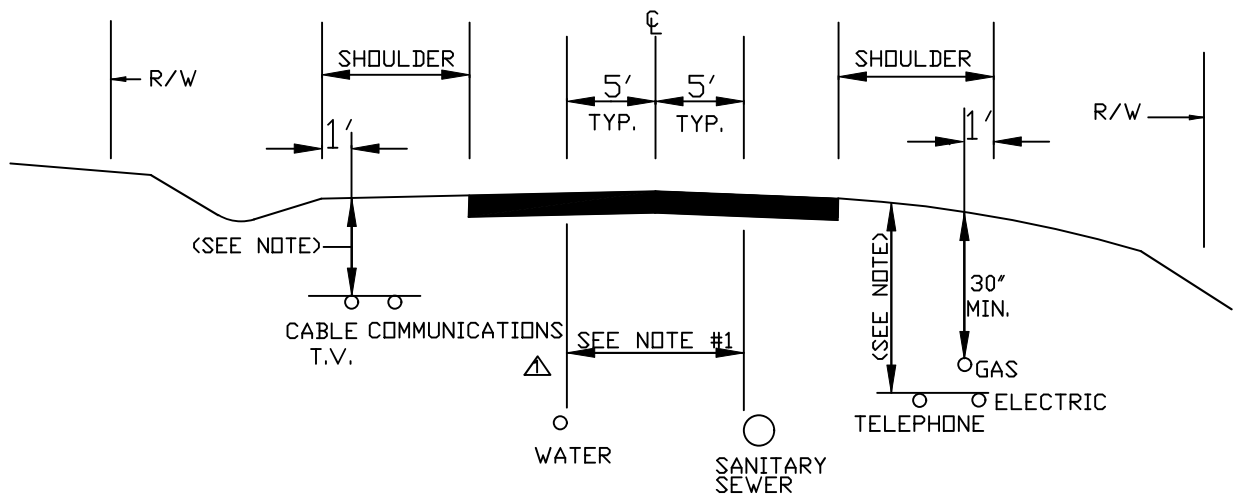
LOCATION OF UTILITIES OPEN SECTION
