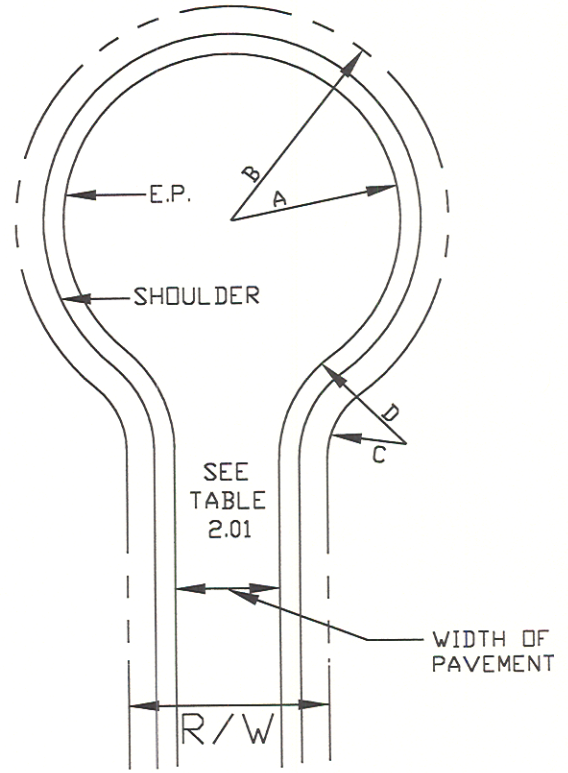
OPEN SECTION
