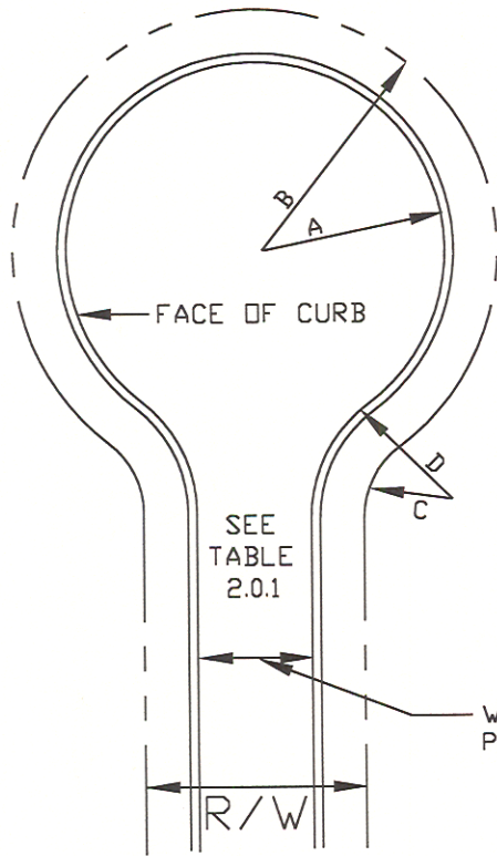
CLOSED SECTION
