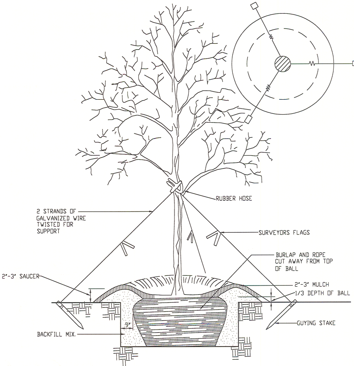
TYPICAL TREE GUYING DETAIL SEE SUPPORT SCHEDULE
