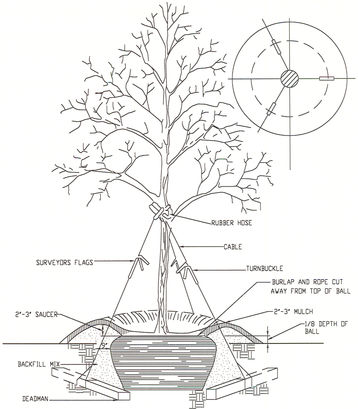
TYPICAL TREE GUYING WITH DEADMEN SEE SUPPORT SCHEDULE
