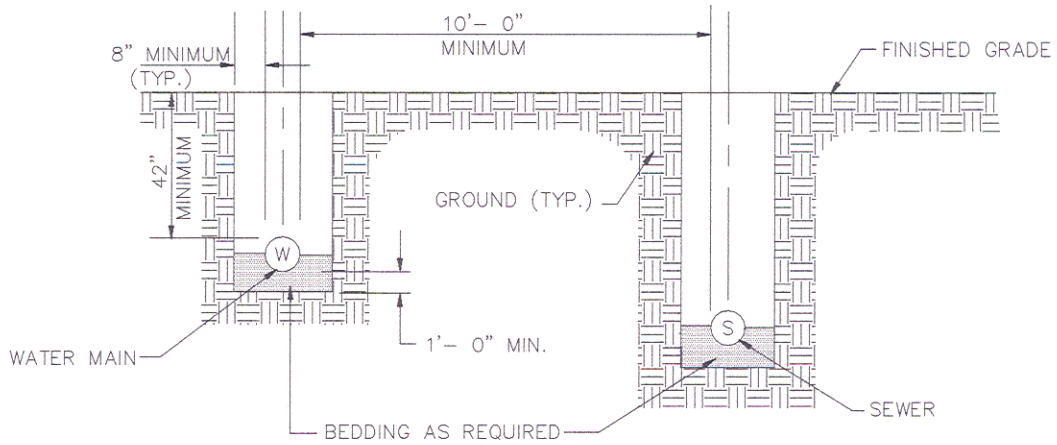
TYPICAL SECTION (SEPARATE TRENCH)
